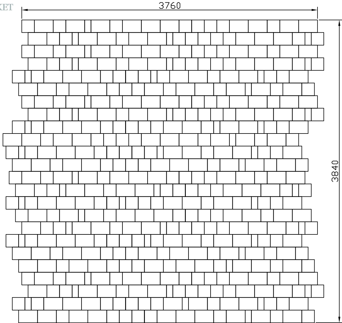
Stretcher Course Pattern (8-15mm nominal joint required)
